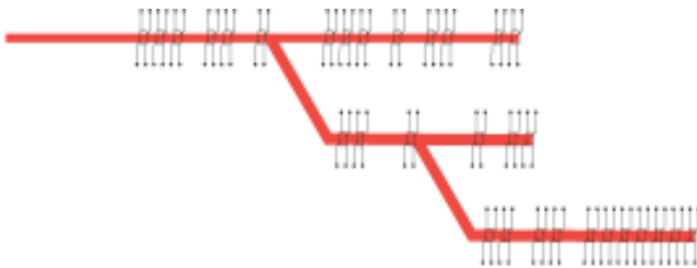
AS-i tree structure
